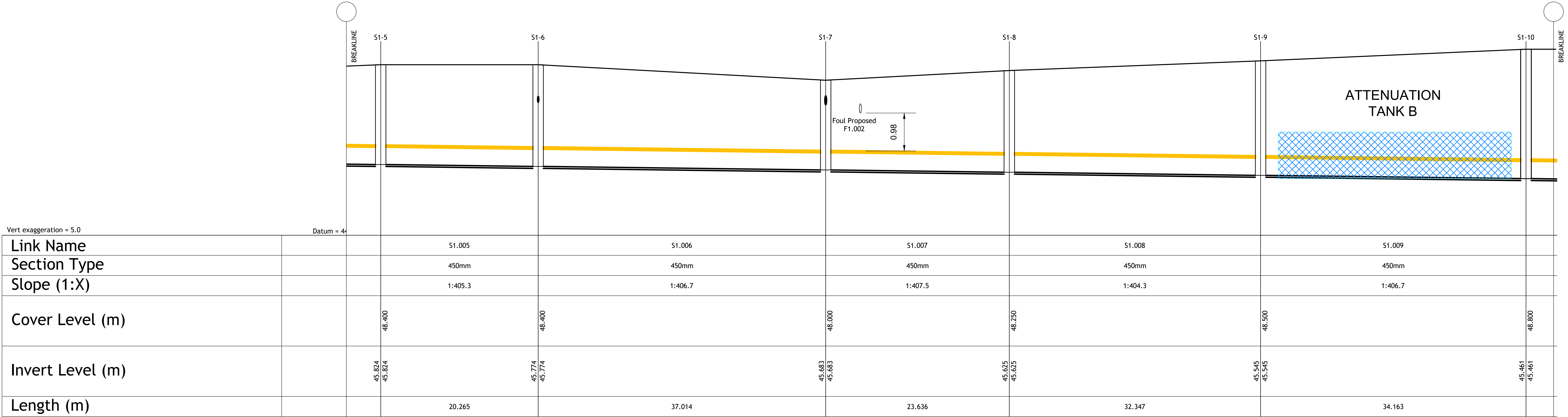
SIC2-0 TO EXT MH4 LONG SECTION - CONTINUATION
