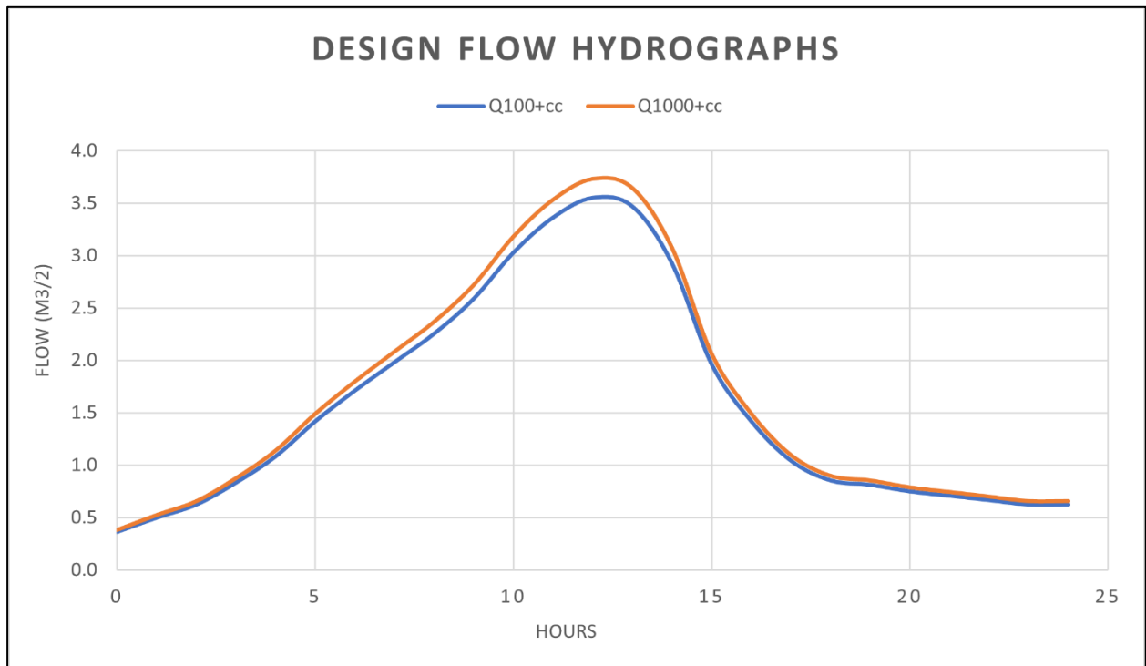
Figure 5-4: Design Flow Hydrographs
