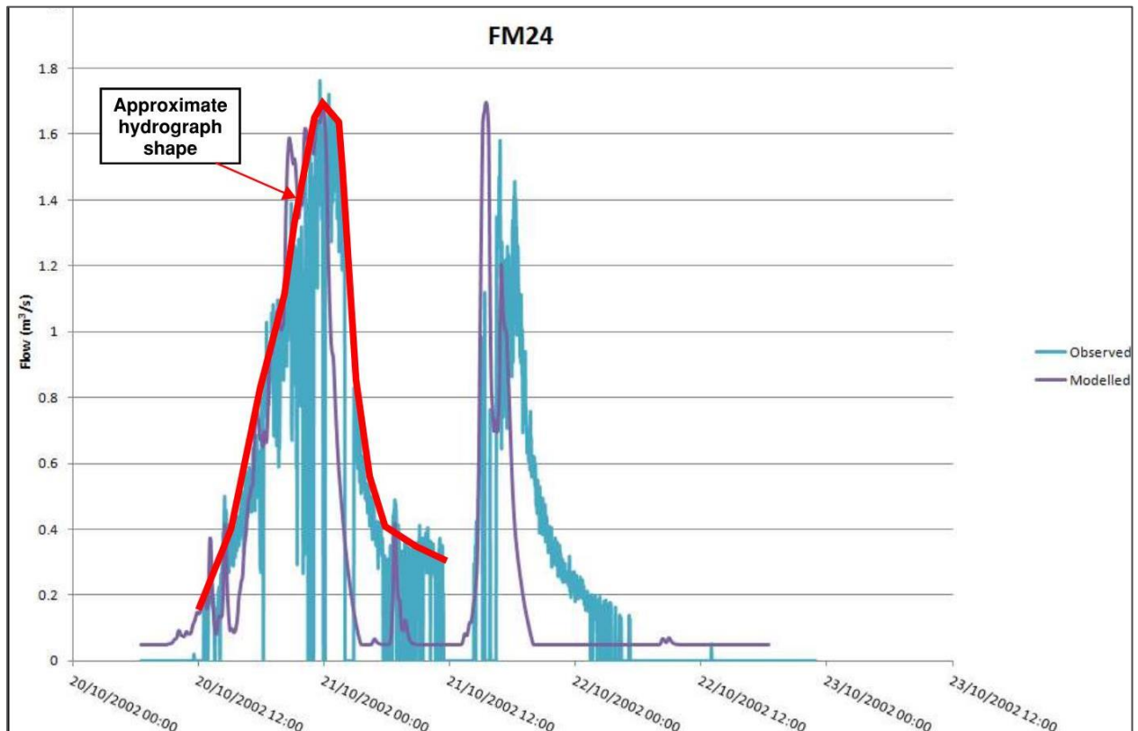
Figure 5-3: Lakelands Overflow Culvert - Recorded Hydrograph (Figure 4.14.18 Eastern CFRAMS UoM09 Hydraulics Report)
