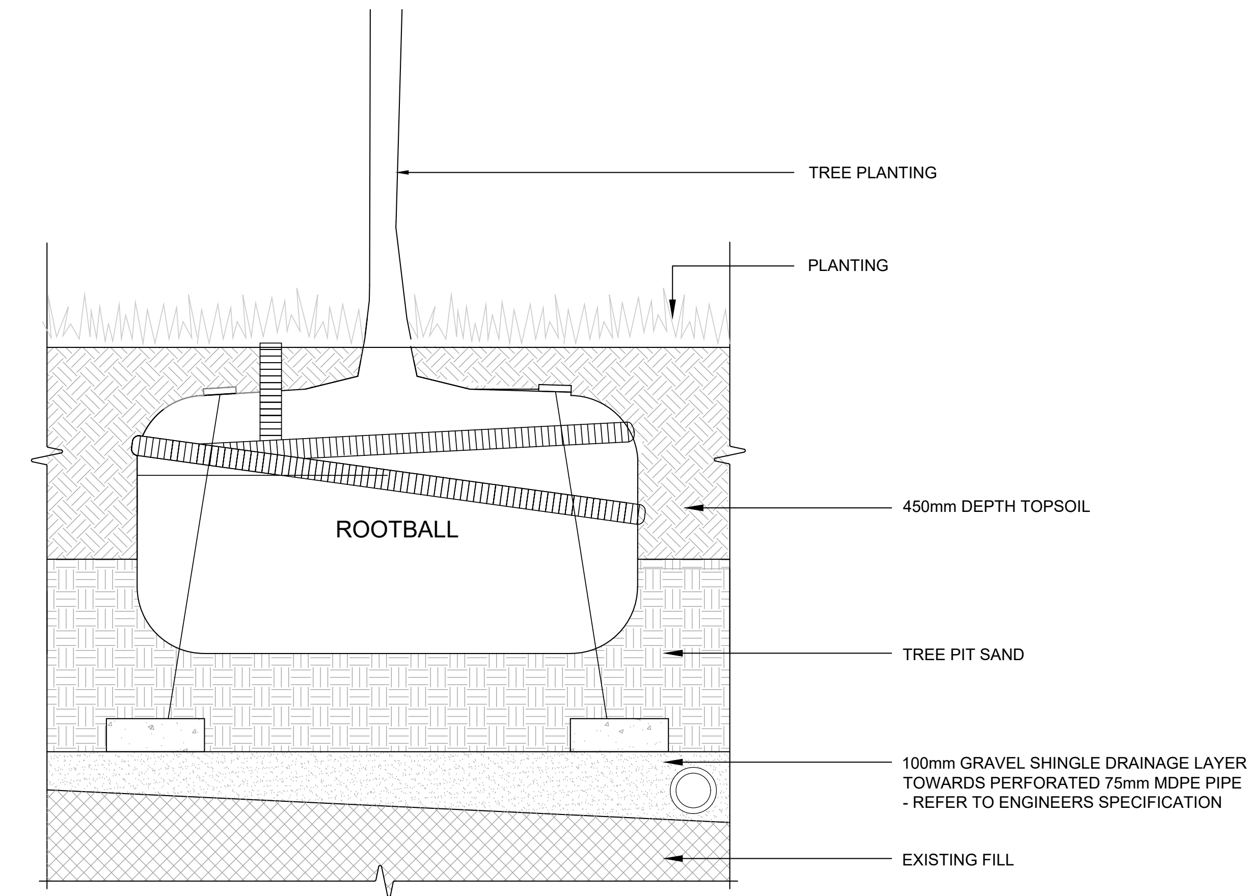
01 TYPICAL DETAIL : TREE PIT SCALE: 1:10 @A1
